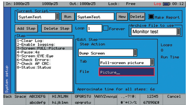
The Command scripts window showing the scripting memories, step list and make report
